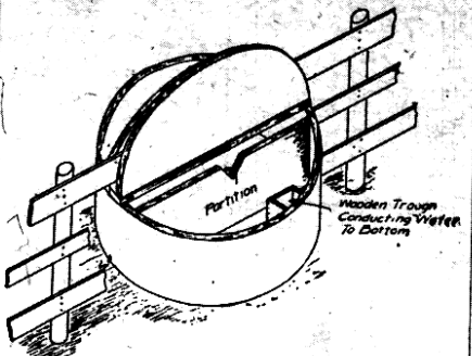
This serves well for a cooling tank. It is the partition water-tight and let the notch carry off the overflow.
