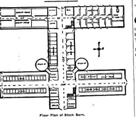
Floor Plan of Stock Barn.
